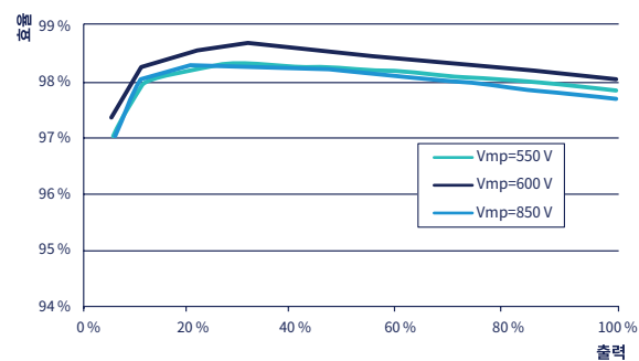
효율곡선(Efficiency Curve)
