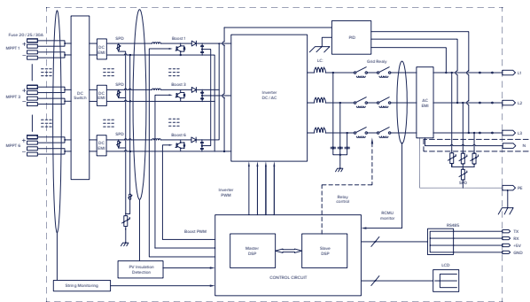
회로도(Circuit Diagram)
